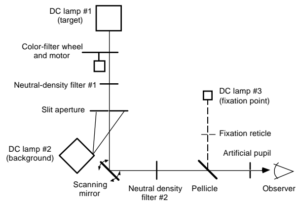
Figure 1. FSC apparatus.
