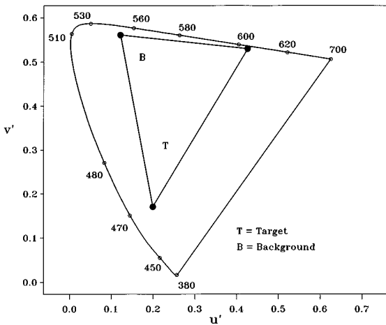
Figure 2. CIE 1976 uniform chromaticity-scale diagram showing the chromaticity coordinates of the FSC system's RGB primaries, the target, and the background.
