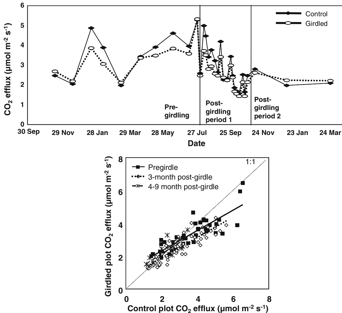
Fig. 3 Soil CO 2 efflux ( upper ) dropped by 15.8% in the first 3 months in response to girdling ( p=0.01 ), but the 6.6% reduction that occurred from 4 to 9 months post-girdling was not significant ( p>0.5 ). The slopes of the relationships between control and
